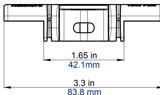
Flush grid (35% open area) top view
