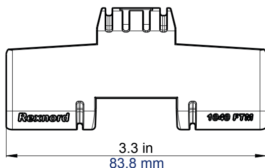
Flat top (closed surface) top view
