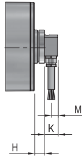
Cable connection 90°
